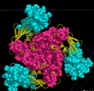
A Constructed Trimers of MP2 and ABT Dimers
