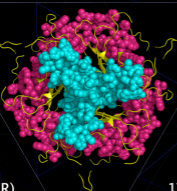
G TMEV-1 VP1 MP2/CRABP Cores and Toxin Cores
